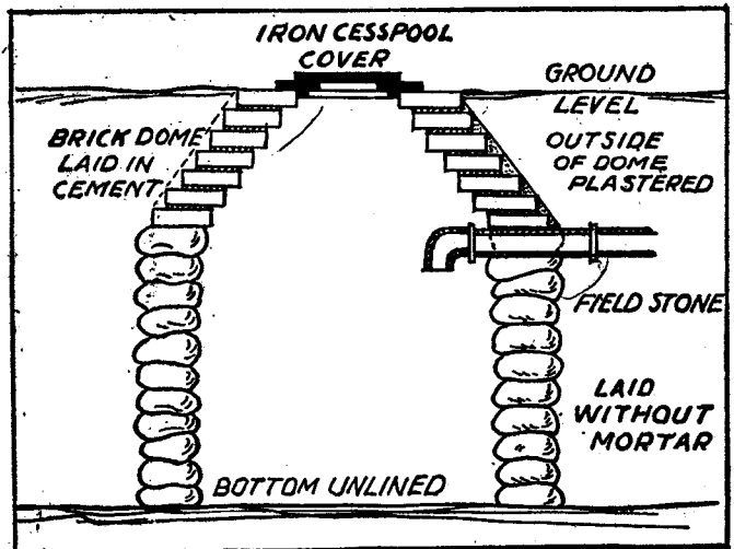
Diagram of cesspool
