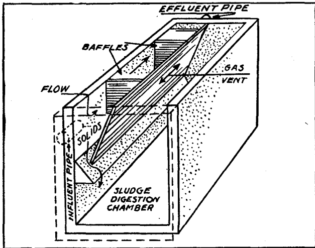
SMALL IMHOFF TANK
